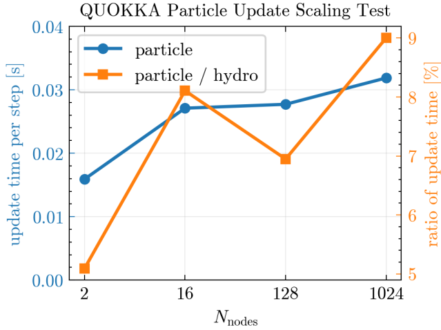
Figure 8. Weak-scaling test of the particle update in QUOKKA for a Milky Way-like disk galaxy simulation. The left y axis shows the wall-clock time for the particle update per coarse step, and the right y axis shows this time expressed as a fraction of the hydrodynamic update time, both as a function of the number of Frontier nodes. We find 50% weak scaling efficiency from 2 to 1024 nodes.
