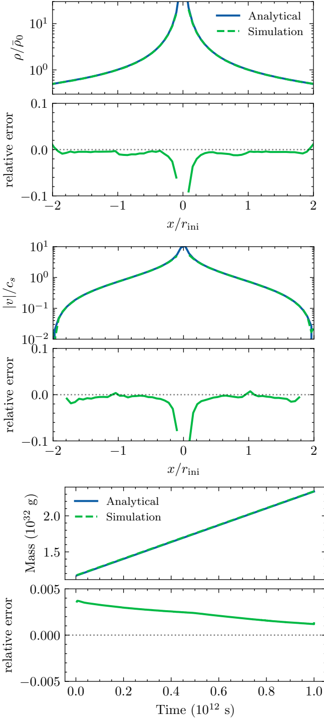
Figure 2. Isothermal sphere test. The top two panels show the mean density and radial velocity as a function of radius in the simulation (dashed green line) compared to the analytic solution (blue solid line). The lower panel shows the sink particle mass versus time, again comparing the simulation and exact analytic solutions.
