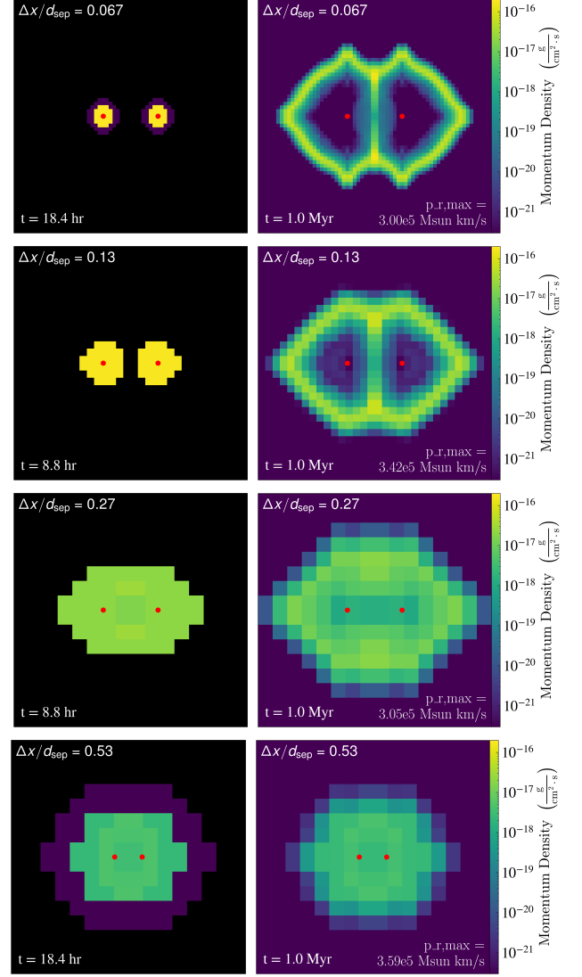
Figure 7. Same as Figure 6 but for a setup where R_{\text{shell}}/d_{\text{sep}} = 0.3 (corresponding to an ambient density n_{\text{H,amb}} = 10 \text{ cm}^{-3} ). The full simulation box is 256 pc in length, but for improved visibility the first three rows are cropped to a 128 pc region. In this configuration, shell formation occurs before SNRs begin to interact. Our numerical method demonstrates convergent terminal radial momentum across spatial resolutions, with discrepancies within 20%.
