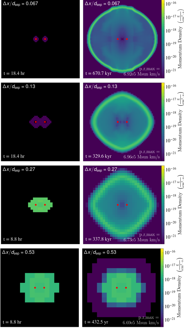
Figure 6. Slices showing radial momentum density in the double-SN test with r_{\text{sf}}/d_{\text{sep}} \approx 2.0 (corresponding to ambient density n_{\text{H,amb}} = 0.1 \text{ cm}^{-3} ), so shell formation occurs only after the two SNRs begin to interact. Red circles mark the locations of the two SNe. The left column shows the configuration after the first time step, immediately after SN deposition, while the right column shows the state at the end of the simulation when the radial momentum has ceased increasing, at the time indicated. Spatial resolutions are 2 pc, 4 pc, 8 pc, and 16 pc, from top to bottom. Our numerical method demonstrates converging results for the terminal radial momentum (see labels at bottom-right corner of the second column) as we vary the spatial resolution.
