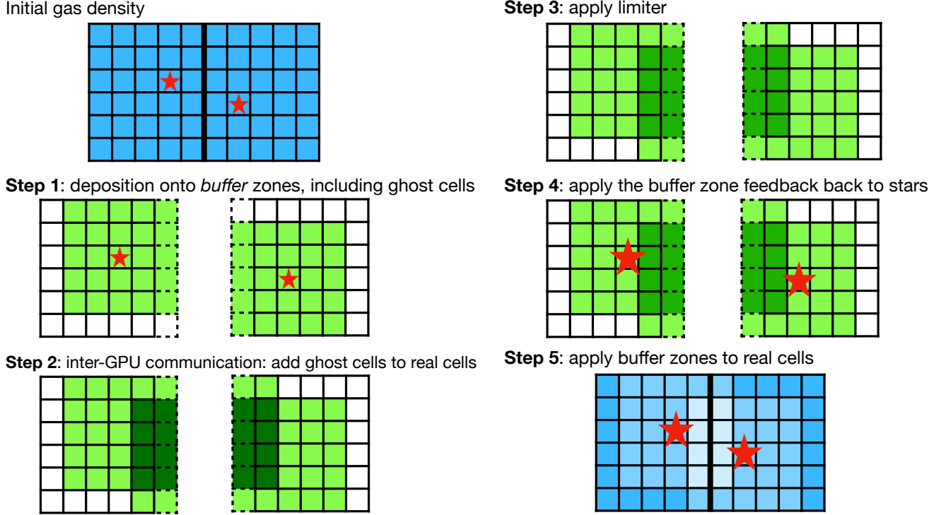
Figure 1. Summary of the steps in the particle-mesh-particle algorithm for particle-gas interactions on GPU. In the example shown, there are two particles (red stars) located near the boundaries of two grids stored in memory on different GPUs; the thick black line indicates the boundary. Blue colouring shows real cells, while green indicates the buffer. Cells with dashed edges are ghost zones used for communication; we show only one ghost zone in this schematic for compactness, but real calculations use a larger number.
