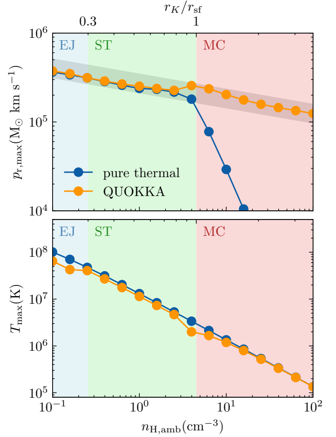
Figure 5. Tests of SN feedback prescriptions using simulations of radiative SNR evolution in a uniform medium with spatial resolution \Delta x = 4 pc, both using our fiducial prescription (orange) and a scheme that deposits thermal energy only (blue). The top panel shows the final radial momentum, while the bottom shows the maximum temperature attained during the simulation, both shown as functions of the ambient hydrogen number density. The grey stripe in the upper panel indicates the empirical p_{r,\text{max}} - n_{\text{H,amb}} relation with 25% tolerance. The upper axis shows the ratio of kernel radius ( = 3\Delta x ) to the shell-formation radius, and the background shading indicates which case of our fiducial SN deposition scheme is used for each simulation given that ratio.
