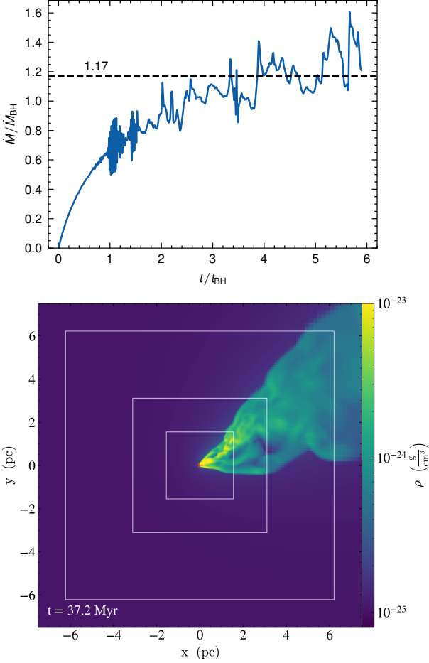
Figure 4. Top: Accretion rate versus time for the Bondi-Hoyle accretion test described in Section 4.3. The accretion rate is normalized to the Bondi-Hoyle accretion rate, and the time is normalized to Bondi-Hoyle time. Bottom: Snapshot of the density field in the xy -plane at t \approx 6t_{\text{BH}} . White squares indicate the borders of the AMR levels.
