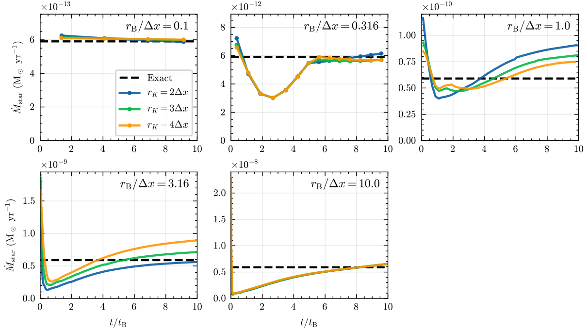
Figure 3. Comparison of simulated accretion rates over time with theoretical values for the Bondi accretion tests presented in Section 4.2. The ratios of the Bondi radius to spatial resolution are, from left to right and top to bottom, 0.1, 0.32, 1.0, 3.16, and 10. The dashed horizontal line denotes the theoretical accretion rate, and the solid lines show the accretion rate measured in the simulations. The horizontal axis gives time in units of the Bondi time.
